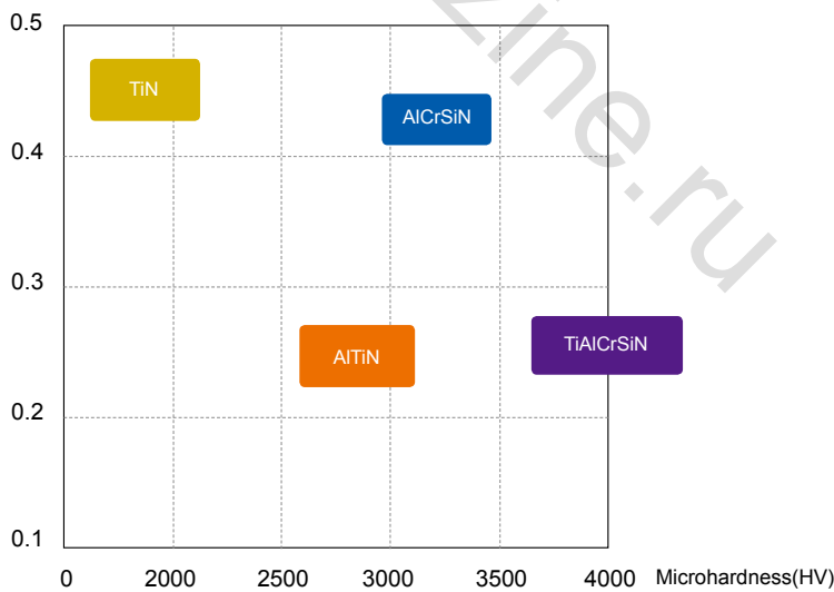
Microhardness and Coefficient of Friction
